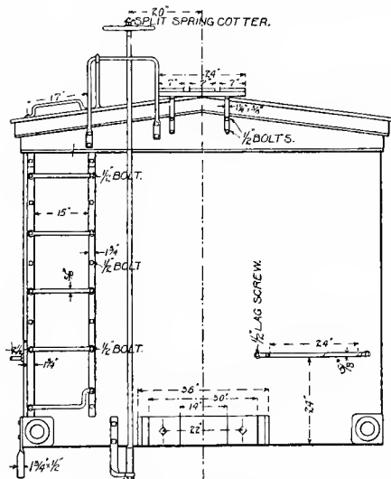
Fig. 5546. End Elevation. POSITIONS AND DIMENSIONS OF BRAKE SHAFT, RUNNING BOARDS, LADDER AND HANDHOLDS.
